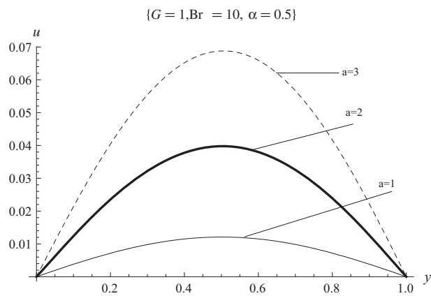
Figure 2 Effect of couple stress inverse parameter on the velocity profile.
