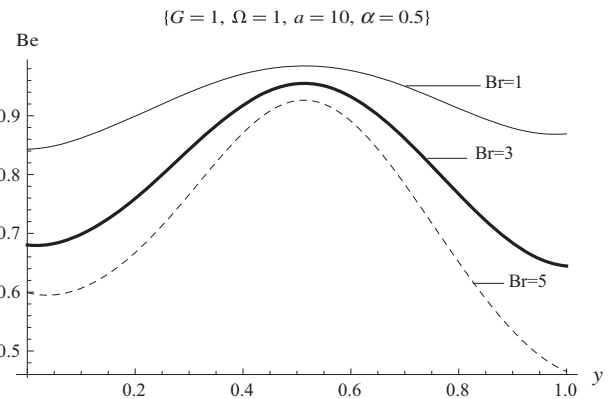
Figure 12 Effect of Brinkman number on irreversibility ratio.
