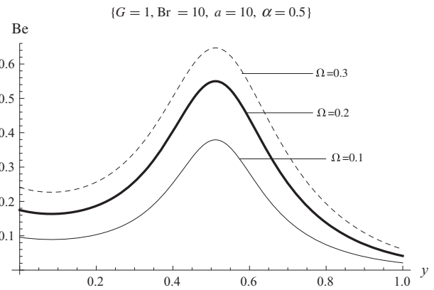
Figure 11 Effect of temperature difference parameter on irreversibility ratio.
