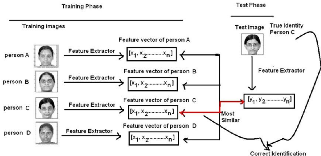
Figure 3: Training and testing phases using PCA for face recognition ([Mee13])
