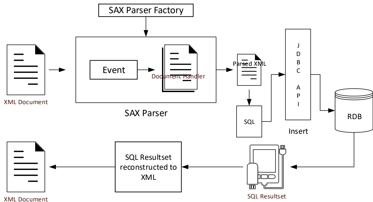
Figure 3. The XAPP architecture.
