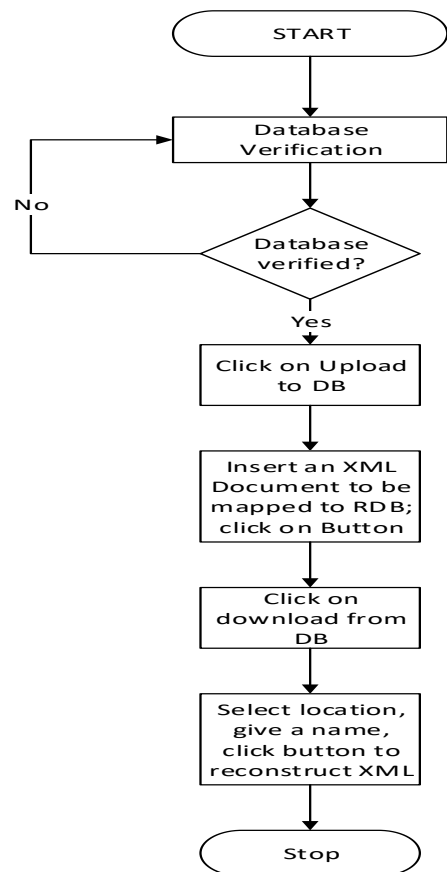
Figure 2. System flowchart of XApp.
