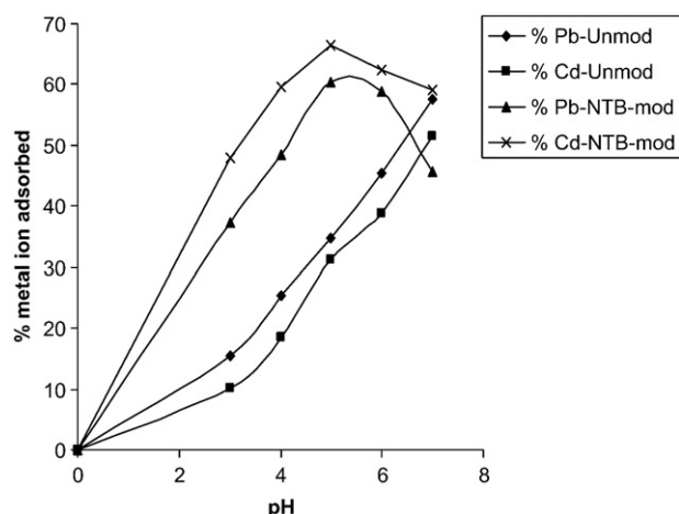
Fig. 8. Effect of pH on the adsorption of Pb (II) and Cd (II) onto unmodified and NTB-modified kaolinite clay samples.
