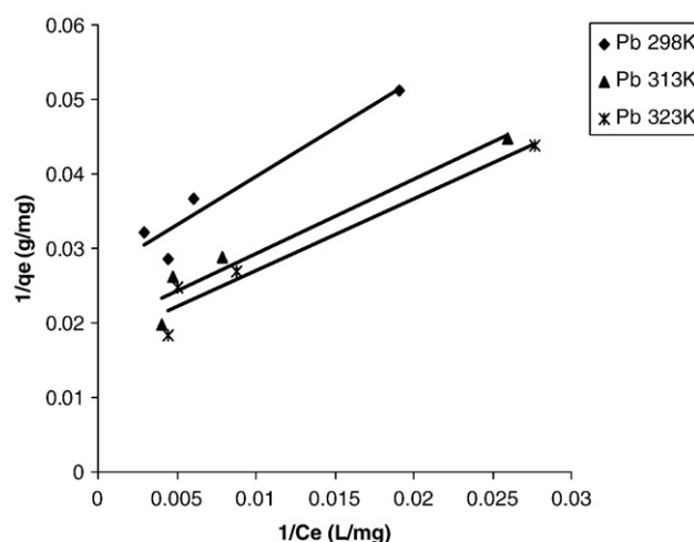
Fig. 9. Langmuir plots for the adsorption of Pb (II) onto unmodified kaolinite clay at various temperatures.
