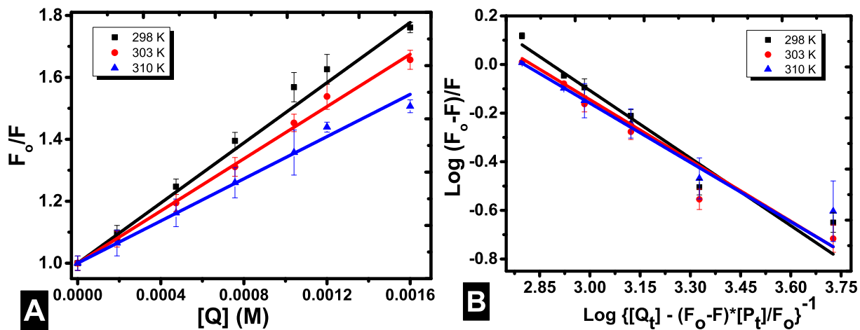
Fig. 2. Stern-Volmer (A) and modified Stern-Volmer (B) plots for the quenching of alpha-amylase by citric acid at three different temperatures, \lambda_{ex} = 280 nm, \lambda_{em} = 300–450 nm, and pH 7.4.
