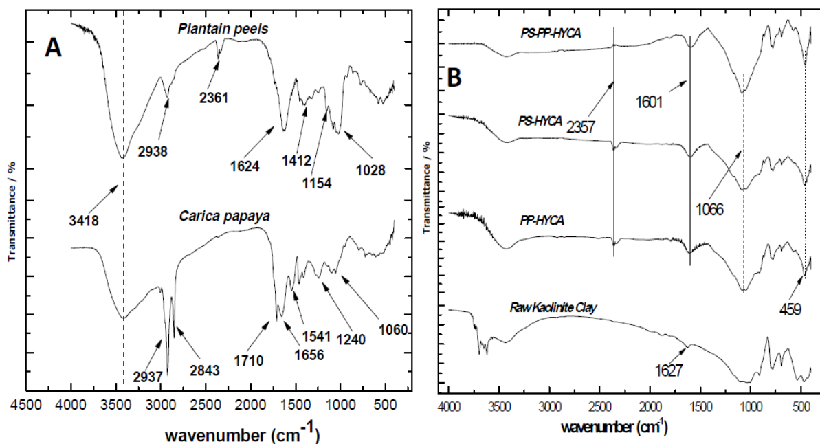
Figure 1. Fourier Transformed Infrared Spectra of (A) Carica papaya seeds and Musa paradisiaca (Plantain) peels (B) kaolinite, Carica papaya -kaolinite (PS-HYCA) and plantain peel-kaolinite (PP-HYCA), Carica papaya -plantain peel-kaolinite (PS-PP-HYCA) composite adsorbents.
