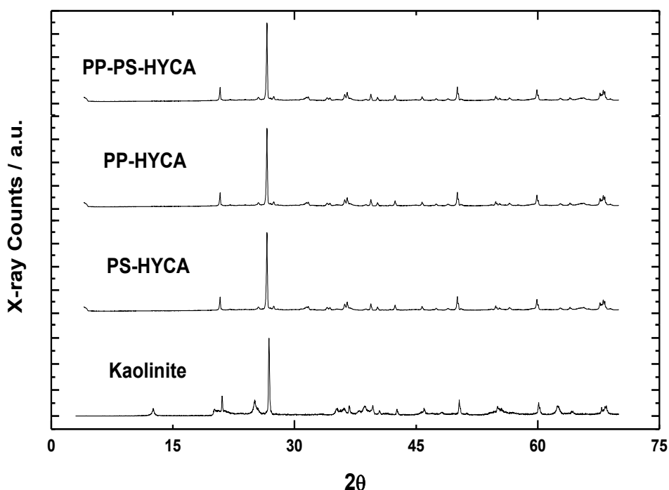
Figure 1c. X-ray Diffraction pattern for Kaolinite, PS-HYCA, PP-HYCA and PS-PP-HYCA composite adsorbents.
