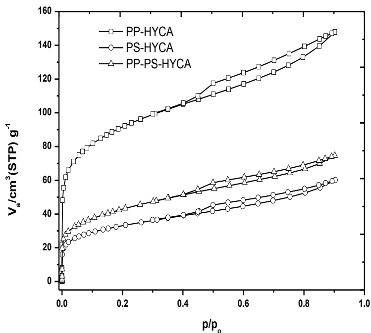
Figure 3. N 2 adsorption/desorption isotherms (77.4 K) for composite adsorbents prepared via microwave @ 540 W for 10 min.
