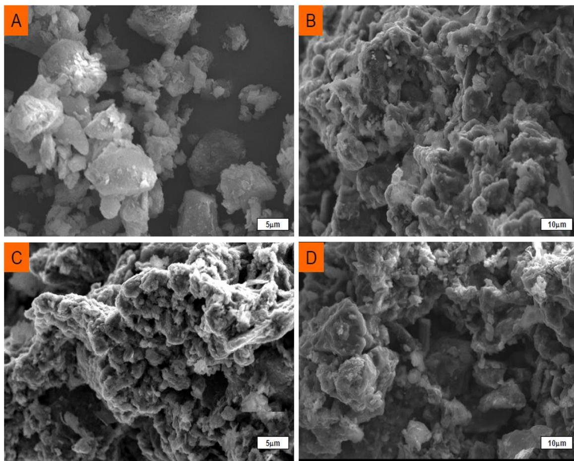
Figure 2. Scanning Electron Microscopy Images of (A) Kaolinite (B) PP-HYCA = plantain peel-Hybrid clay composite adsorbent;(C) PS-HYCA = Carica papaya seeds-Hybrid Clay composite adsorbent (D) PS-PP-HYCA = Papaya seeds-Plantain peel-Hybrid Clay composite adsorbent (Plantain Peel = Musa spp. )
