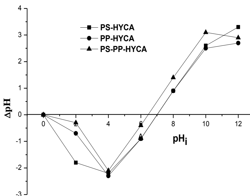
Figure 8: pH_{pzc} of PP-HYCA, PS-HYCA and PS-PP-HYCA composite adsorbents.
