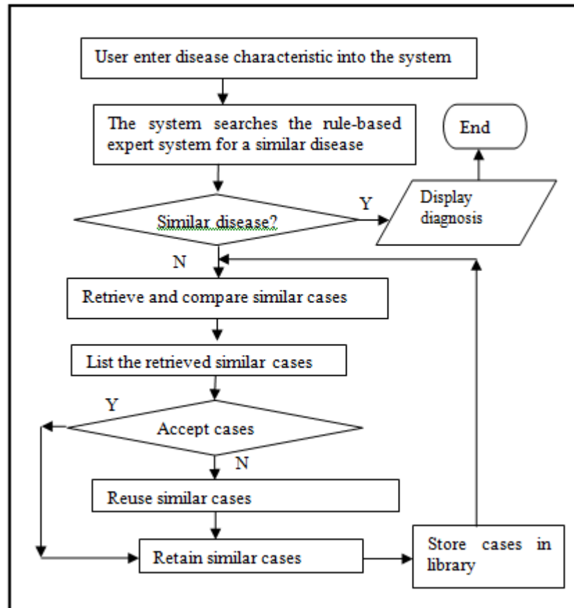
Fig. 4: Flow of data in the integrated architecture for HDBD
