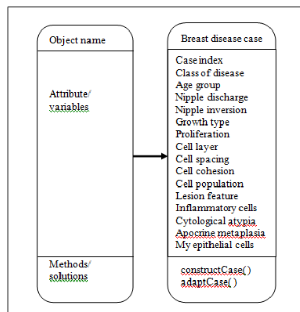
Fig. 2: Structure of Objects
