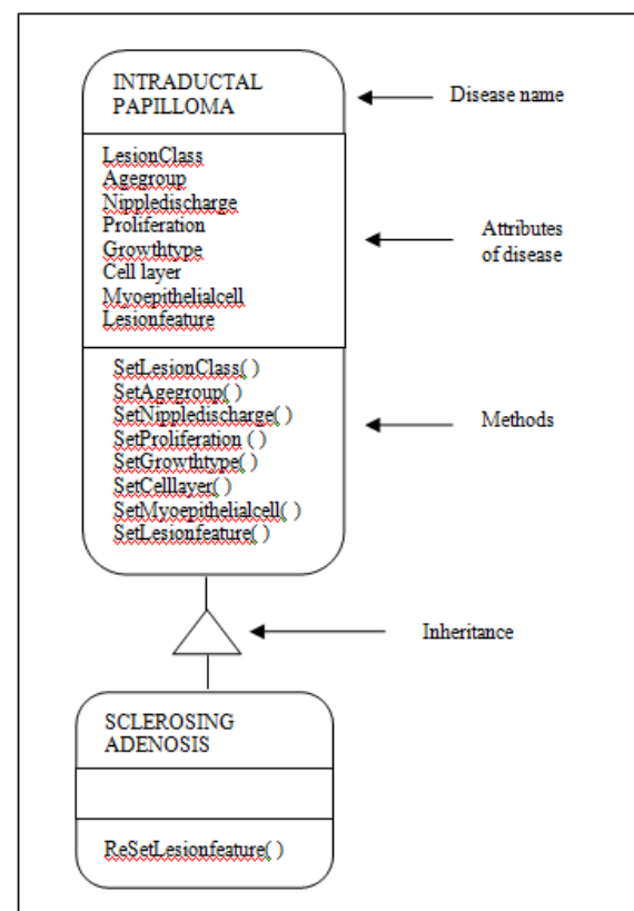
Fig. 5: Inheritance in objects.
