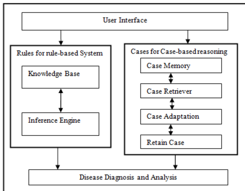
Fig. 3: Integrated architecture for HDBD
