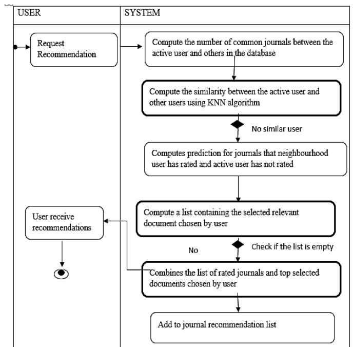
Figure 2: The Hybrid Filtering Recommendation Activity Diagram
