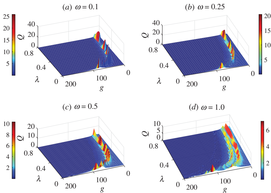
Figure 1. Typical vibrations of a position-dependent mass system driven by dual-frequency forces showing the appearance of resonance peaks taking the form of ridge-shaped ‘hills’, stretching along the mass nonlinearity parameter values \lambda , and spreading across the two planes. The response of the system was numerically computed as a function of the strength of mass nonlinearity \lambda and the high-frequency signal amplitude g for different values of the low-frequency \omega [16]. (Online version in colour.)
