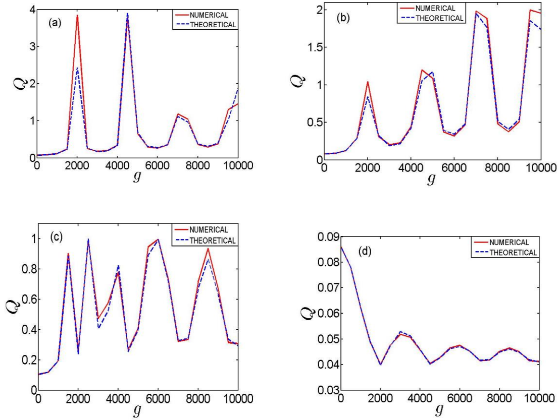
Fig. 3: (Colour online) Evolution of response amplitude, Q , versus amplitude of high signal, g with: (a) \omega = 1.0 ; (b) \omega = 1.5 ; (c) \omega = 2.0 and (d) \omega = 2.4 and other parameters fixed at b = 0.5 , f = 0.1 , \omega = 2 , \gamma_1 = 1.6 , \gamma_2 = -0.867 , \gamma_3 = 3.24 . The continuous lines represent numerically generated Q_{num} from Eq. (23) while the broken lines represent the corresponding analytical values computed from Eq. (21).
