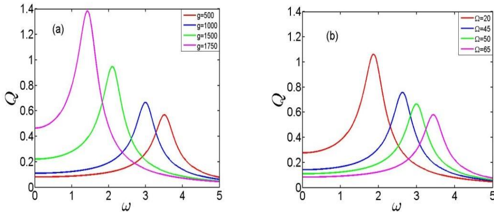
Fig. 4: (Colour online) Frequency response of the system with different values of g and \Omega with other parameters fixed at b = 0.5 , f = 0.1 , \omega = 2 , \gamma_1 = 1.6 , \gamma_2 = -0.867 , \gamma_3 = 3.24
