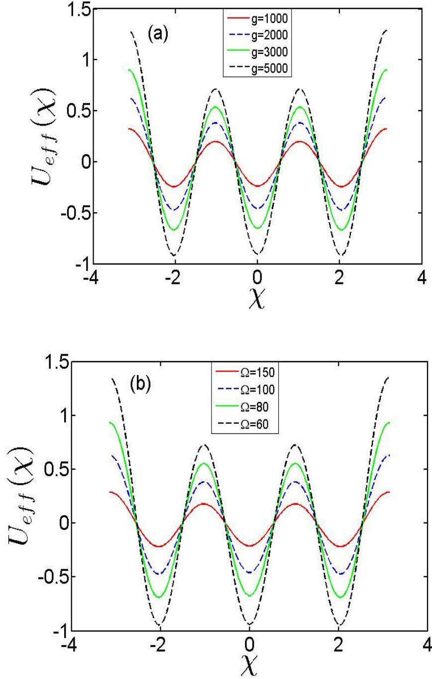
Fig.2: (Colour online) The shape of effective potential against \chi with the following parameters: b = 0.5 , \gamma_1 = 1.6 , \gamma_2 = -0.867 , \gamma_3 = 3.24 ; and \omega = 2 .
