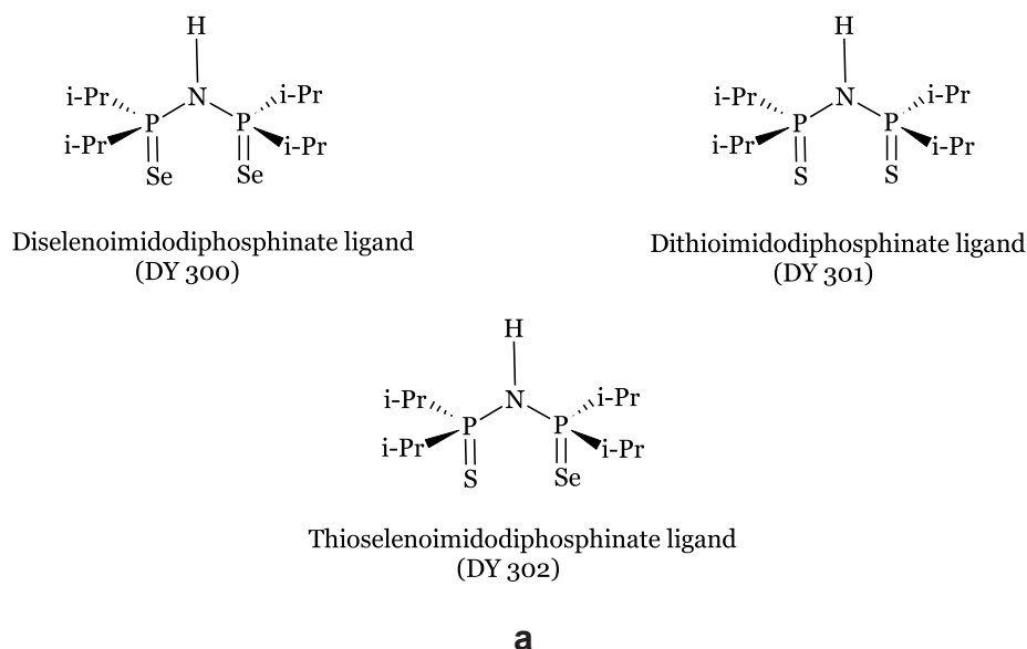
Fig. 1a. Structures of dichalcogenoimidodiphosphinate ligands (DY300, DY301 and DY302) investigated in the present study.
