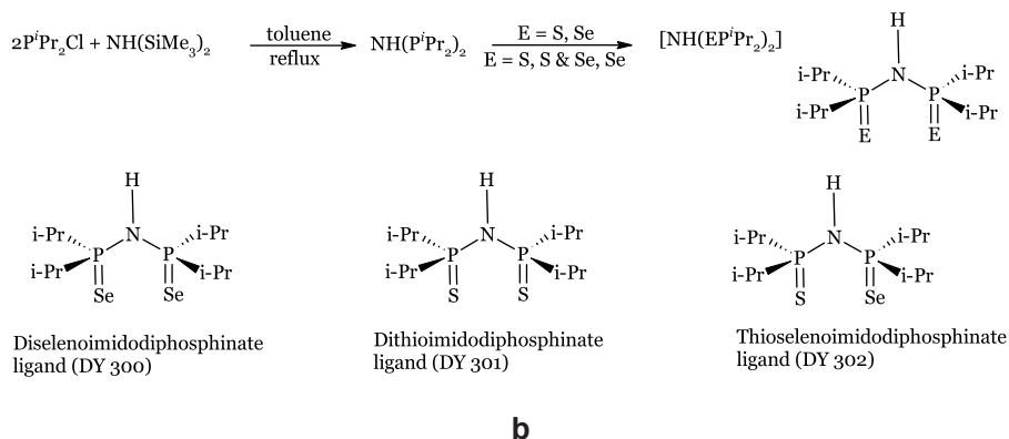
Fig. 1b. Reaction scheme for the synthesis of dichalcogenoimidodiphosphinate ligands.
