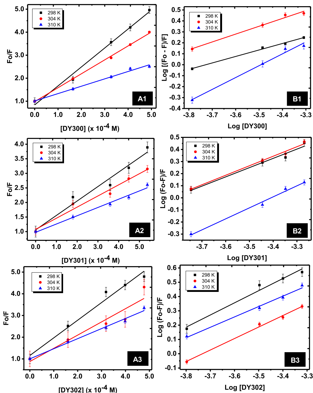
Fig. 4. Stern-Volmer (A) and modified Stern-Volmer (B) plots for binding interactions between \alpha -amylase and dichalcogenoimidodiphosphinate ligands (DY300, DY301 and DY302) at pH 6.8 under different temperature conditions (298, 304 and 310 K).
