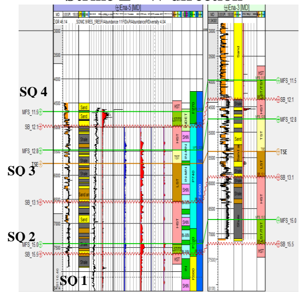
Figure 3b: Cross section of Ena-5 and Ena-3 on the strike direction
