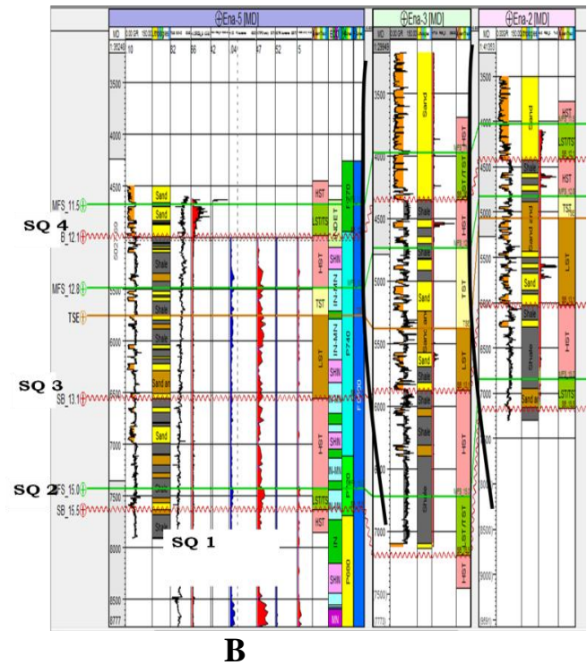
Figure 2b: Cross section of Ena-5, Ena-3 and Ena-2 dipping direction.
