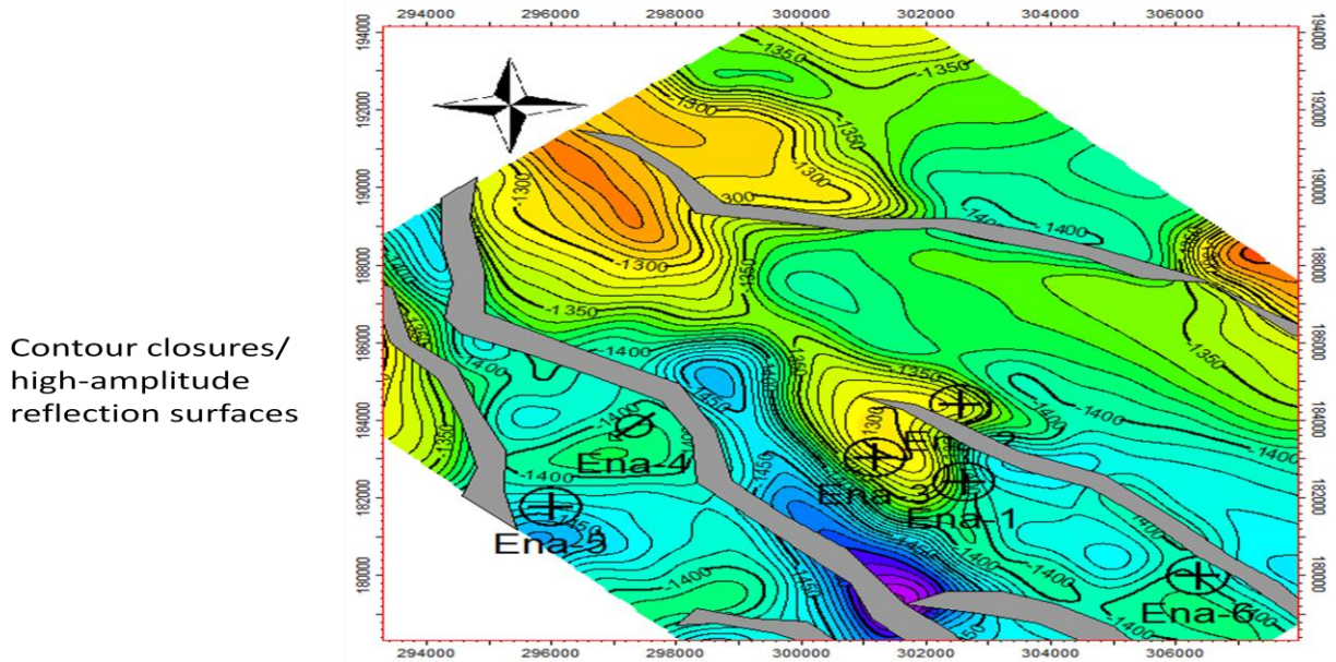
Figure 6: MFS 12.8Ma surface with up dip areas is an implication of hydrocarbons.
