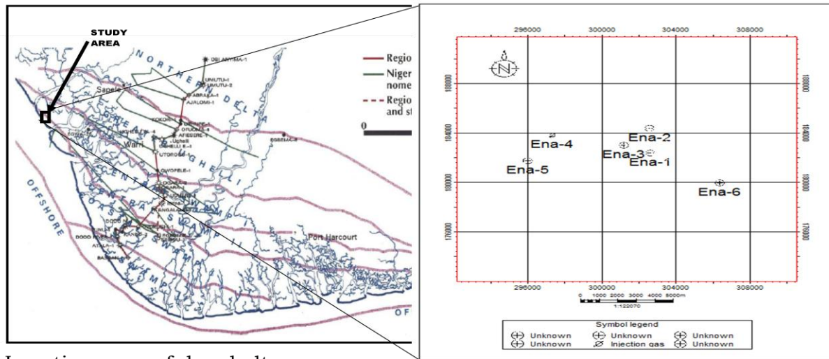
Location map of depobelts, (after Reijers, 2011)
