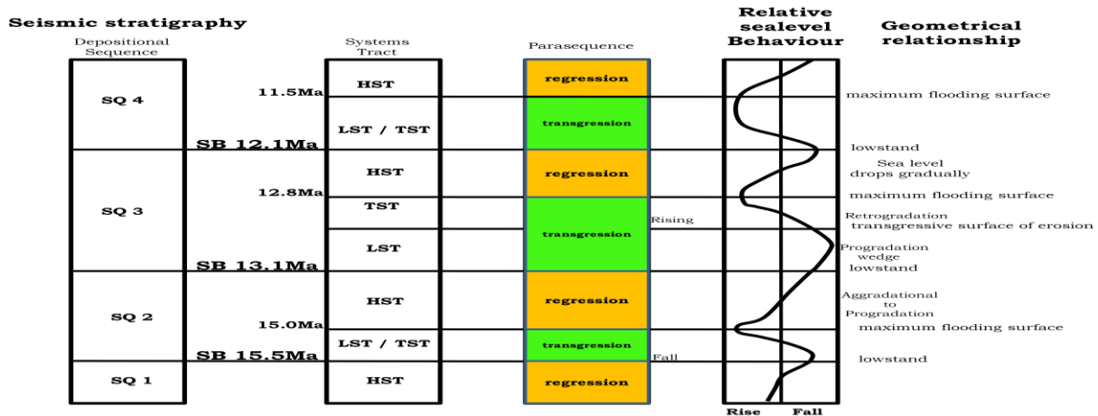
Figure 4: Schematic Seismic parameters within the third-order sequences and their systems tracts.
