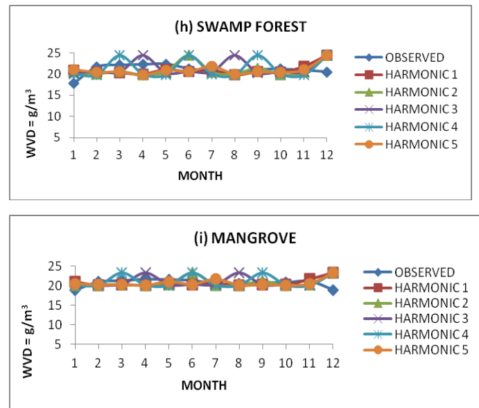
Figure 4: Monthly mean values and amplitudes of first five harmonics of water vapour density.
