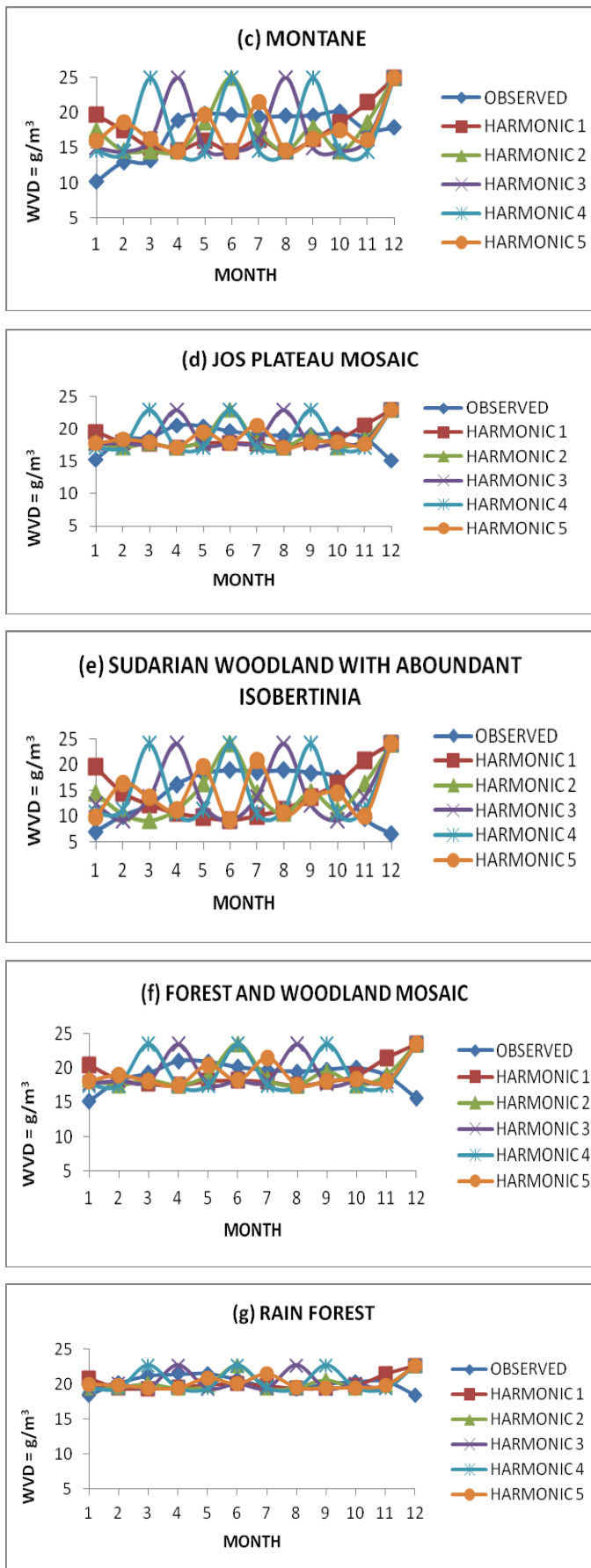
Figure 4: Monthly mean values and amplitudes of first five harmonics of water vapour density.
