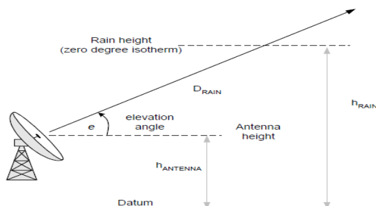
Figure 3: A schematic diagram of earth-space showing the slant range of the portion of the signal that lies below the freezing point ( ITU-R 2003).
