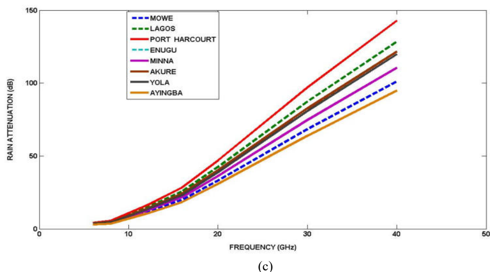
Figure 7: Attenuation at 0.01% exceedance for all regions for (a) vertical polarization, (b) horizontal polarization, and (c) circular polarization.
