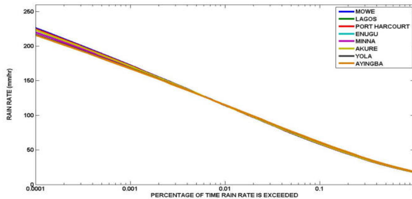
Figure 5: Combined rain rate for the eight TRODAN stations at percentages of exceedance.
