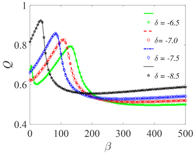
Fig. 11. Plot of the response amplitude Q versus \beta with varying \delta = -6.5, -7.0, -7.5 and -8.5 ; for f = 10, \omega = 6.5, \epsilon = 0.01, \lambda = 145, \Omega = 10\omega and \gamma = -329 . Continuous curves or broken lines represent the numerically-computed Q from Eq. (19) using Eq. (42), while the analytically calculated Q from Eqs. (34) and (42), are indicated by marker points.
