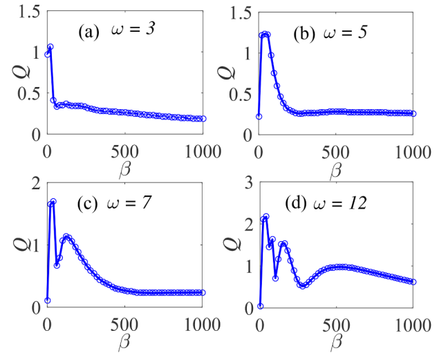
Fig. 13. Dependence of Q on \beta for (a) \omega = 3 (b) \omega = 5 (c) \omega = 7 and (d) \omega = 12 with \Omega = 20\omega, f = 20, \lambda = 145, \epsilon = 0.01, \eta = 1.5 , and \gamma = -32.9 . Continuous curves represent the numerically-computed Q from Eq. (19) using Eq. (42), while the analytically calculated Q from Eqs. (34) and (42), are indicated by marker points and/or broken lines.
