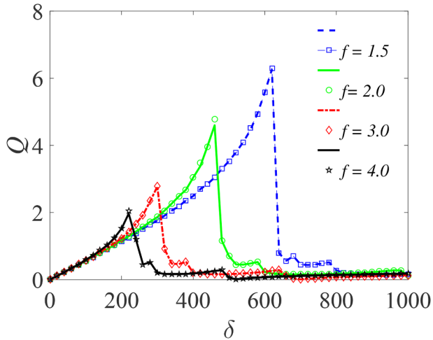
Fig. 12. Plot of the response amplitude Q versus \delta the effective contribution of the ambient pressure to the acoustic sound field, with by amplitude of the fast signal f = 1.5, 2.0, 3.0 and 4.0 ; for \Omega = 30\omega, \omega = 5, \epsilon = 0.01, \beta = -474, \lambda = 145, \eta = 1.50 and \gamma = -32.9 . Continuous curves or broken lines represent the numerically-computed Q from Eq. (19) using Eq. (42), while the analytically calculated Q from Eqs. (34) and (42), are indicated by marker points.
