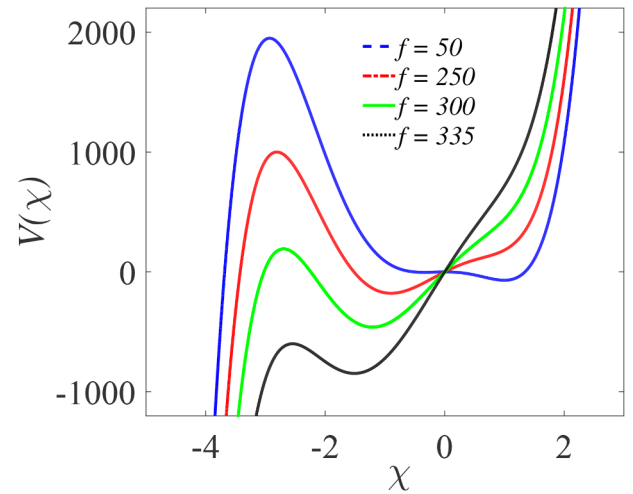
Fig. 4. The effective potential of the system computed from Eq. (31), with four values of f ( =50, 250, 300, 335 and 300 ) and other parameters are \beta = \lambda = 145 , \delta = -10 , \Omega = 10\omega , \omega = 5 , \epsilon = 1 , and \gamma = -329 with t = 10^6 .
