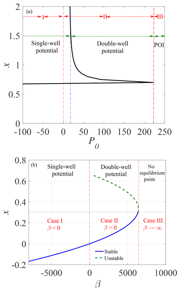
Fig. 1. The dependence of the non-dimensional bubble radius x on; (a) the ambient pressure P_0 and (b) \beta the resonance frequency of the system.
