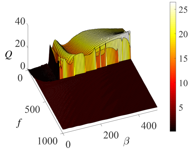
Fig. 14. Surface plot of Q as a function of f and \beta for \omega = 20, \Omega = 15\omega, \lambda = 100, \epsilon = 0.01, \eta = 1.5 , and \gamma = 400 .
