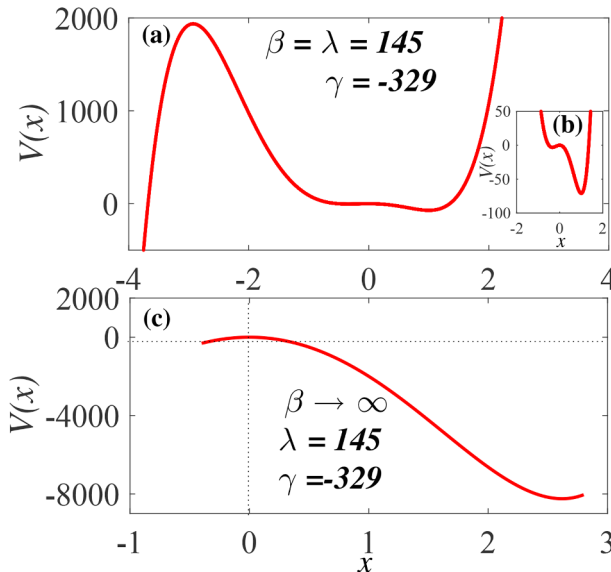
Fig. 3. The bubble oscillator potential V(x) from Eq. (14): (a) double-well for \beta > 0 , \gamma < 0 and \lambda > 0 , (two stable equilibria and two unstable equilibria). The parameters are \lambda = 145 and \gamma = -329 . (b) Zoom of the asymmetric double-well potential in (a). (c) Point of no equilibrium with other parameters fixed as in (a) for \beta \rightarrow \infty , (point of inflection with \beta = 4000 ).
