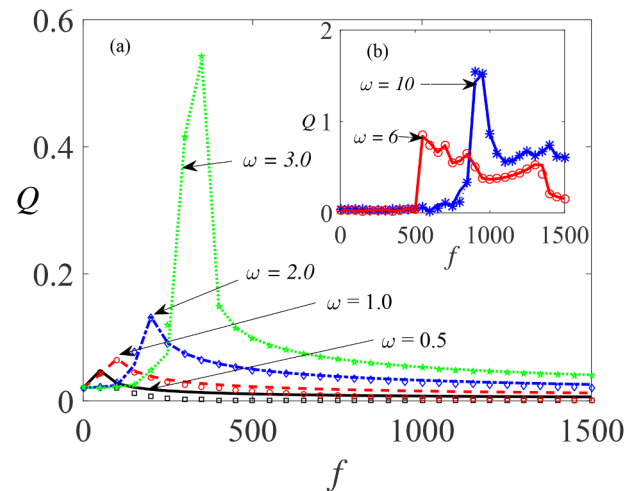
Fig. 6. Response amplitude, Q against f for different values of \omega = 0.5, 1.0, 2.0 , and 3.0 with \Omega = 20\omega , \beta = -245 , \epsilon = 0.01 , \lambda = 145 , \delta = -2 and \gamma = -32.9 . Continuous curves or broken lines represent the numerically-computed Q from Eq. (19) using Eq. (42), while the analytically calculated Q from Eqs. (34) and (42), are indicated by marker points.
