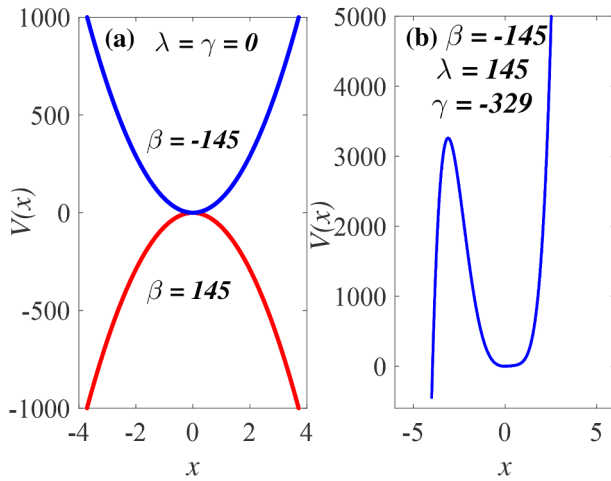
Fig. 2. The bubble oscillator potential V(x) from Eq. (14) for single well conditions: (a) single-well for \beta < 0 , \gamma = \lambda = 0 (a stable equilibrium) and single-hump for \beta > 0 , \gamma = \lambda = 0 (an unstable equilibrium); (b) single-well-single-hump for \beta < 0 , \gamma < 0 and \lambda > 0 , (two equilibria, one unstable and one stable equilibrium). In (b) the parameters are \lambda = 145 and \gamma = -329 .
