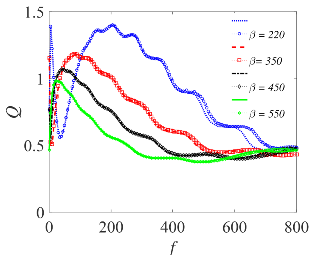
Fig. 8. Dependence of Q on f with varying \beta = 220, 350, 450 and 550 ; for \Omega = 19\omega , \eta = 1.5 , \omega = 12 , \epsilon = 0.01 , \lambda = 145 , \delta = -2 and \gamma = -32.9 . Continuous or broken line represent the numerically-computed Q from Eq. (19) using Eq. (42), while the analytically calculated Q from Eqs. (34) and (42), are indicated by marker points.
