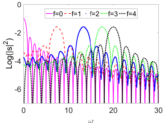
FIG. 3. (Color Online) Resonance peaks in the low-frequency force regime of Tietz-Hua quantum oscillator with negative potential constant, c_h = -0.2 : (a) f = 0 ; (b) f = 1 ; (c) f = 2 ; (d) f = 3 ; (e) f = 4 .
