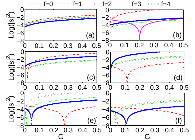
FIG. 6. (Colour online) Quantum vibrational antiresonance (QVAR) in the low-frequency force regime of Tietz-Hua quantum oscillator with positive potential constant, c_h = 0.2 . (a) \omega = 1.0 , (b) \omega = 1.7 , (c) \omega = 2.0 , (d) \omega = 3.0 , (e) \omega = 4.0 , (f) \omega = 5.0
