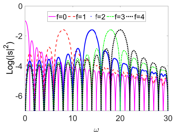
FIG. 4. (Color Online) Resonance peaks in the low-frequency force regime of Tietz-Hua quantum oscillator with zero potential constant, c_h = 0 : (a) f = 0 ; (b) f = 1 ; (c) f = 2 ; (d) f = 3 ; (e) f = 4 .
