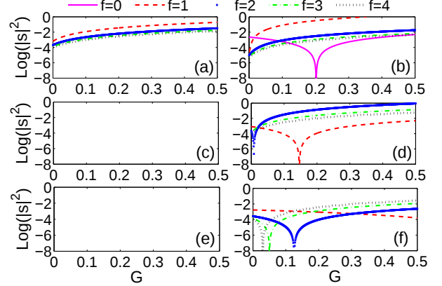
FIG. 5. (Colour online) Quantum vibrational antiresonance (QVAR) in the low-frequency force regime of Tietz-Hua quantum oscillator with zero potential constant, c_h = 0 . (a) \omega = 1.0 , (b) \omega = 1.7 , (c) \omega = 2.0 , (d) \omega = 3.0 , (e) \omega = 4.0 , (f) \omega = 5.0
