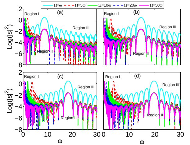
FIG. 8. (Colour online) Effects of high-frequency on |s|^2 in the excited states f = 1, 2, 3 and 4 for different values of \Omega = n\omega scaled as n = 1, 5, 10, 20 and 50 . The other parameters are: c_h = 0.2 , F = 0.05 and G = 0.5 .
