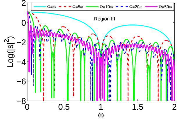
FIG. 7. (Colour online) Effects of high-frequency on |s|^2 in the ground state f = 0 , for different values of \Omega = n\omega scaled as n = 1, 5, 10, 20 and 50 . The other parameters are: c_h = 0.2 , F = 0.05 and G = 0.5
