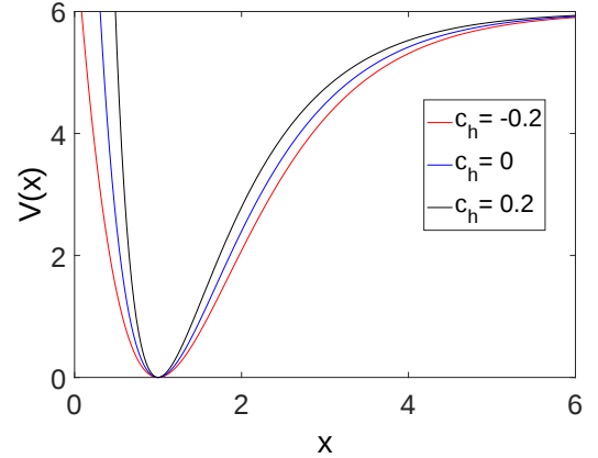
FIG. 1. (Colour online) The shape of the Tietz-Hua potential for the parameters \gamma = 1 , V_0 = 6 and different values of c_h .
