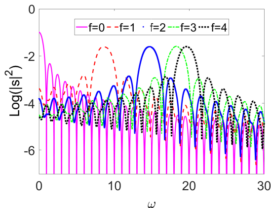
FIG. 2. (Color Online) Resonance peaks in the low-frequency force regime of Tietz-Hua quantum oscillator with positive potential constant, c_h = 0.2 : (a) f = 0 ; (b) f = 1 ; (c) f = 2 ; (d) f = 3 ; (e) f = 4 .
