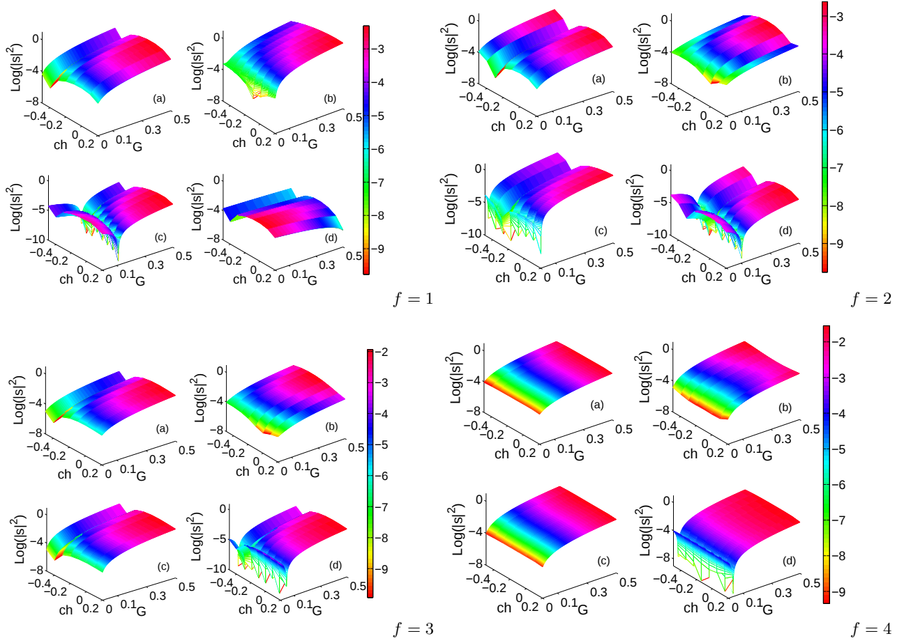
FIG. 10. (Colour online) Three-dimensional view of the transition probability |s|^2 as functions of both c_h and G showing the effects of high-frequency for integer multiples of \Omega ( \Omega = n\omega ), where n = 5 is an integer and g = 0.05 . Subplots labelled (a-d) correspond to different values of the low-frequency \omega fixed as [1, 1.7, 3, 5] . (a) f = 1 , (b) f = 2 , (c) f = 3 and (d) f = 4 .
