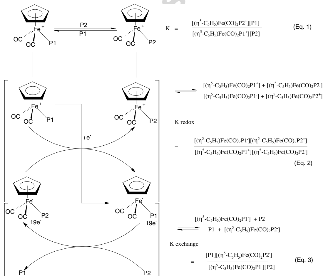
Scheme 1. Phosphine exchange reaction with an electron-transfer chain catalytic pathway.
